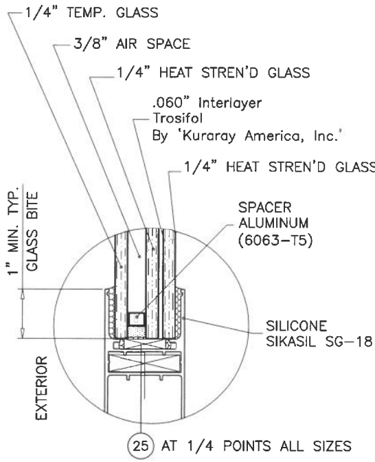
GLASS TYPE 'Ai' 1-3/16" OVERALL INSUL. LAM. GLASS
